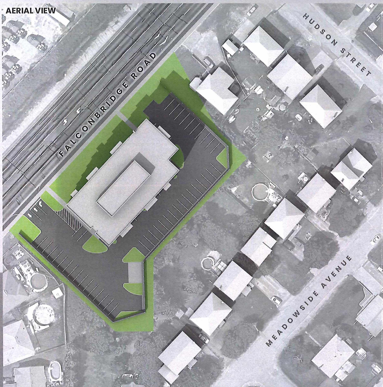
AERIAL VIEW OF 5 STOREY MULTIPLE RESIDENTIAL COMPLEX | AUTUMN EQUINOX SUN SHADOW CASTING ON DWELLINGS TO NORTHEAST BEGINS AT 2:45 PM, SEPTEMBER 22
