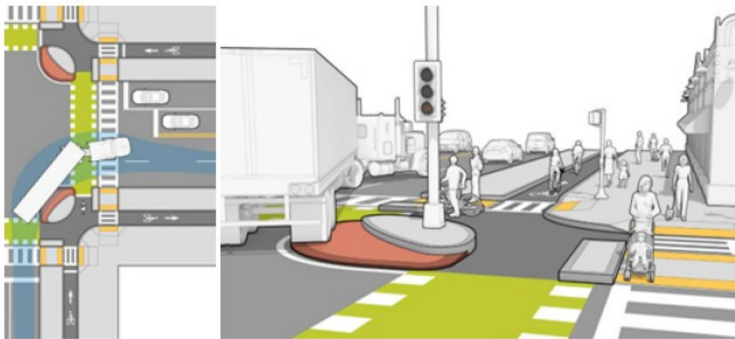
Figure 75. (Left) An overhead view of a mountable truck apron (Right) An on-street view of a truck using the mountable truck apron
